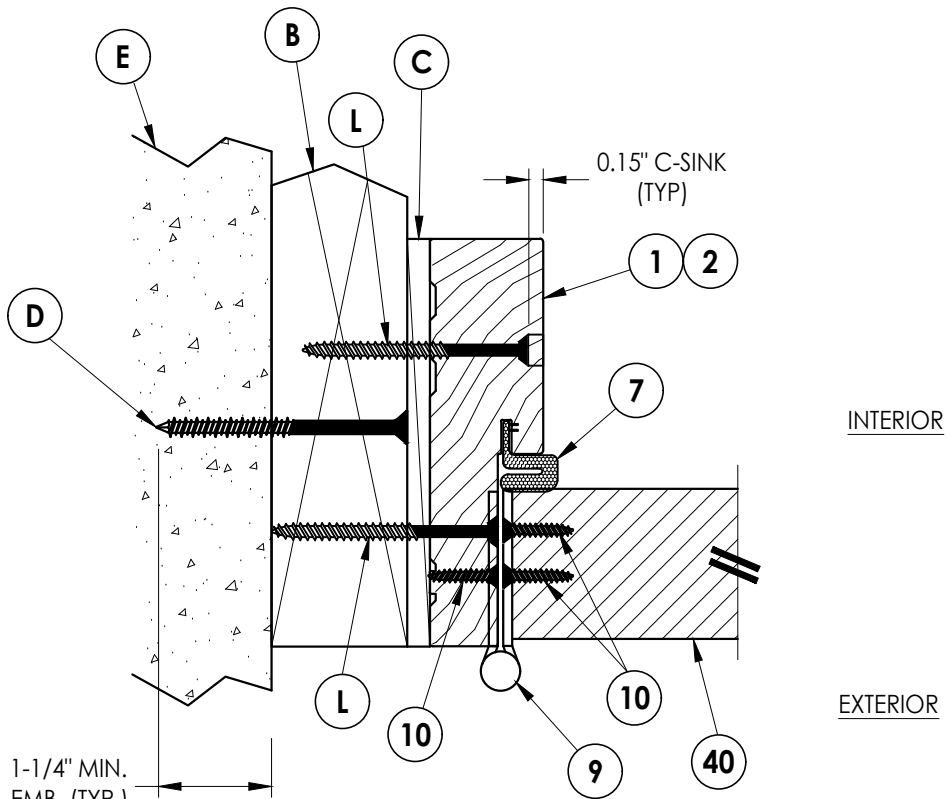
2 3 HORIZONTAL CROSS SECTION Outswing shown (Inswing similar)
