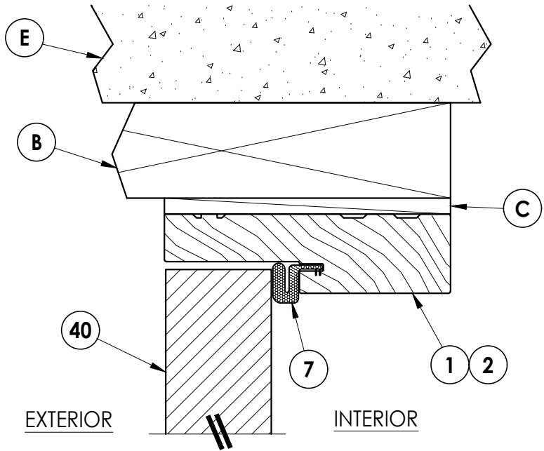
1 3 VERTICAL CROSS SECTION Outswing shown (Inswing similar)
